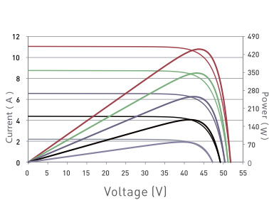
Current-Voltage & Power-Voltage Curves (475W)
